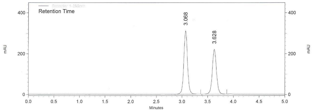
Figure 14 :linearity results of level 120
